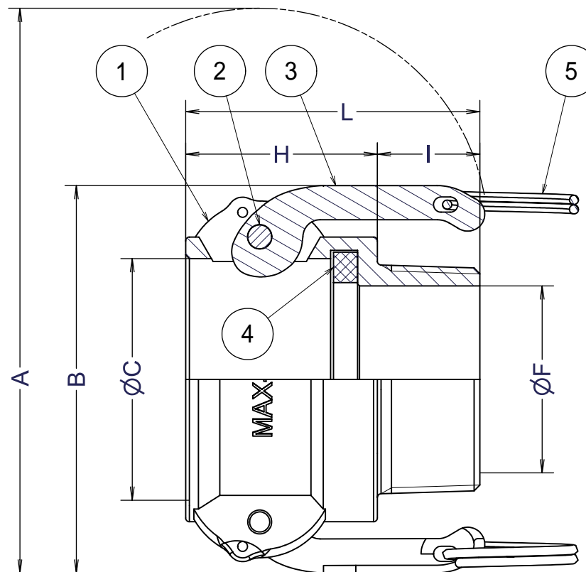
Section C-C
