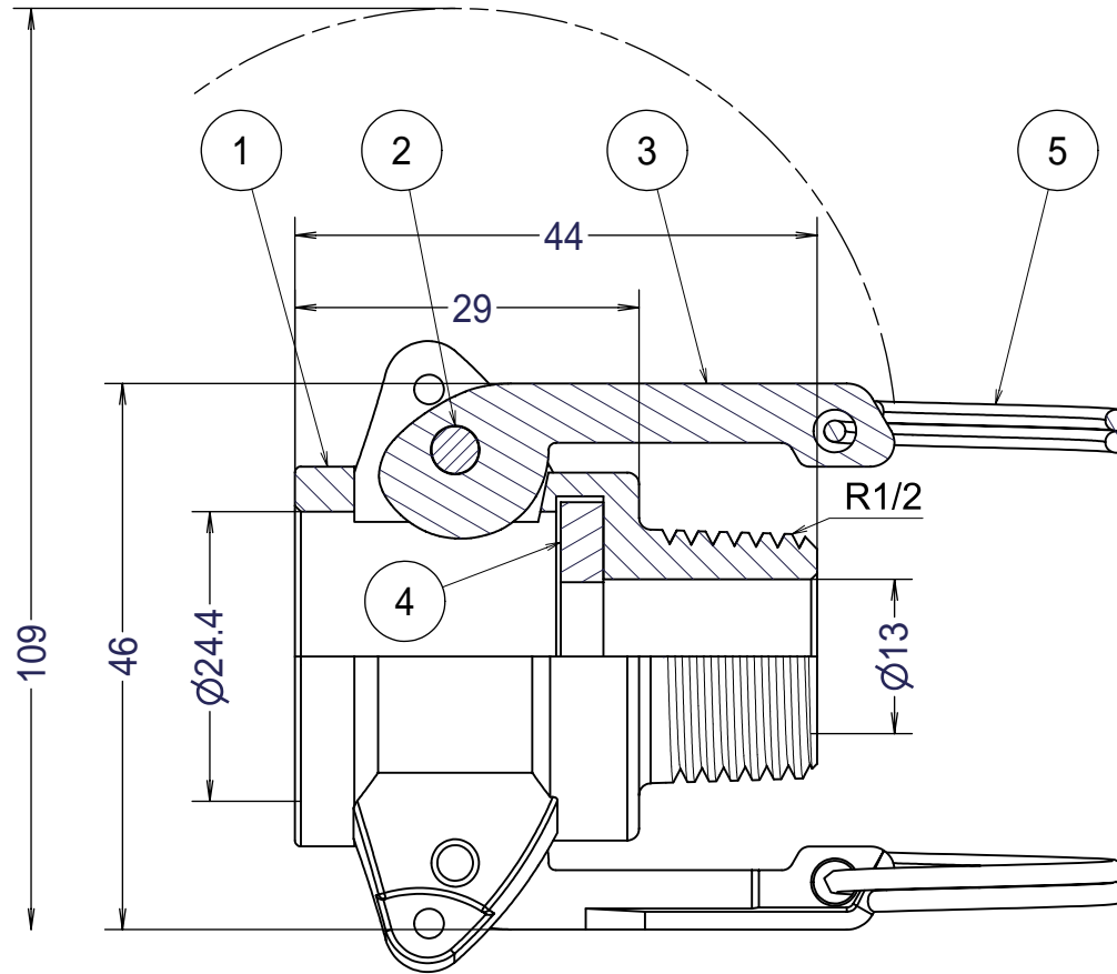
Section C-C
