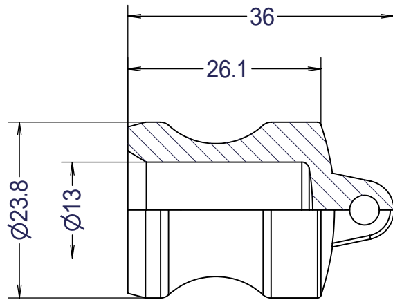
Section E-E
