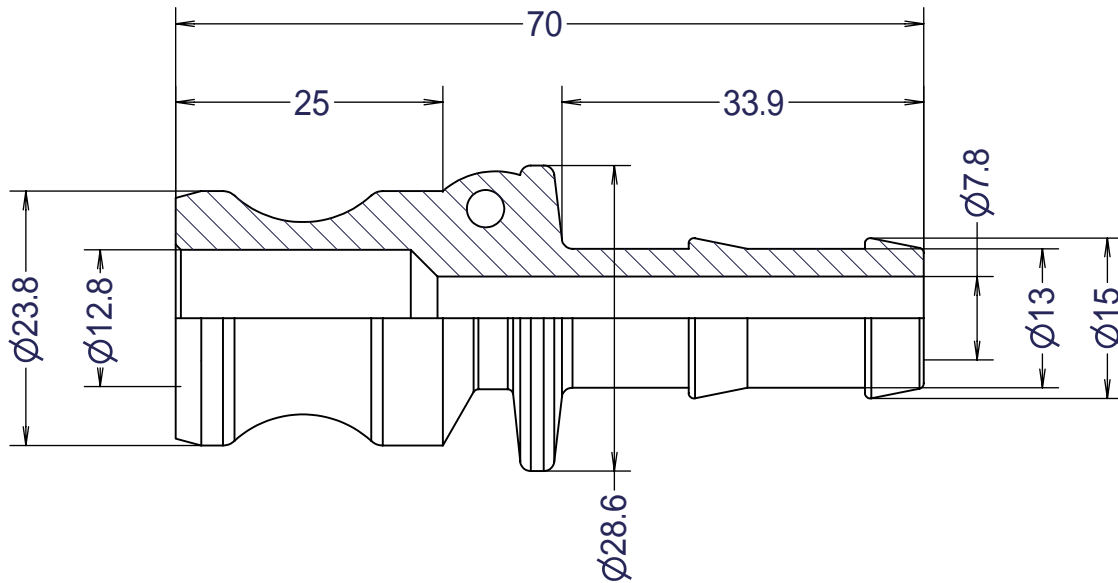
Section E-E
