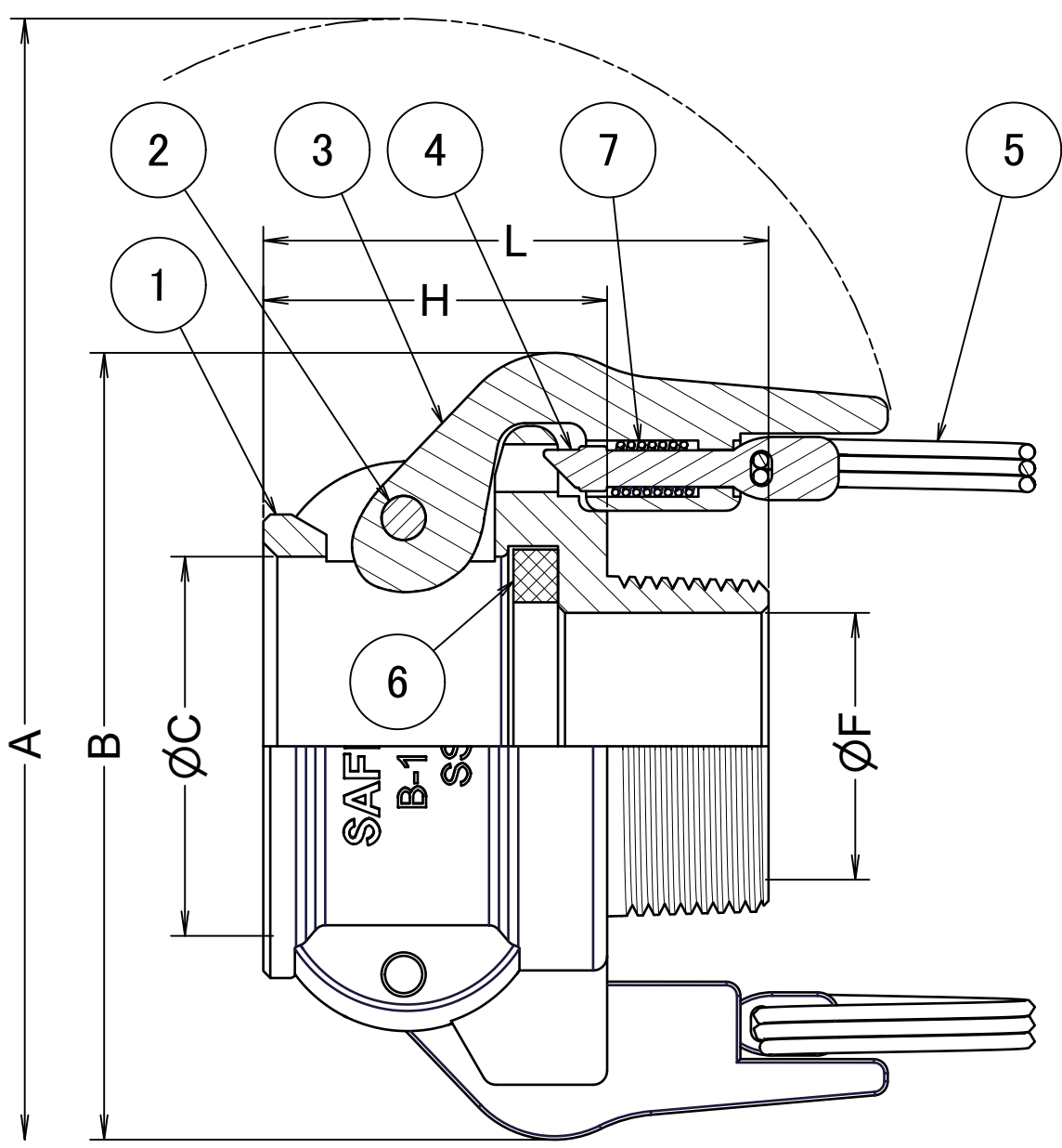
Section F-F
